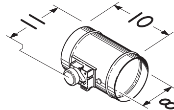
Model MD8T Model SMD8 Model MD8TR
