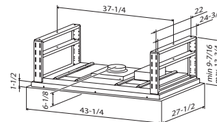
8" Round Duct
