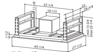
8" Round Duct
