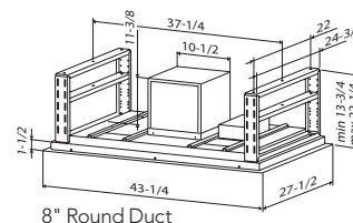
8" Round Duct
