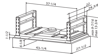
8" Round Duct
